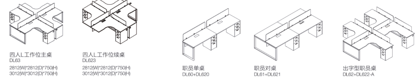
单人职员位续桌 DL620 1200W*1600D*750H 1400W*1600D*750H 1500W*1600D*750H 1600W*1600D*750H 两人工作位主桌 DL61 1200W*1212D*750H 1400W*1412D*750H 1500W*1412D*750H 1600W*1412D*750H 两人工作位续桌 DL621 1200W*1212D*750H 1400W*1412D*750H 1500W*1412D*750H 1600W*1412D*750H 两人L工作位主桌 DL62 1400W*2812D*750H 1500W*3012D*750H 1600W*3212D*750H 两人L工作位续桌 DL622-A 1400W*2812D*750H 1500W*3012D*750H 1600W*3212D*750H 两人L工作位续桌 DL622-B 1400W*2812D*750H 1500W*3012D*750H 1600W*3212D*750H
